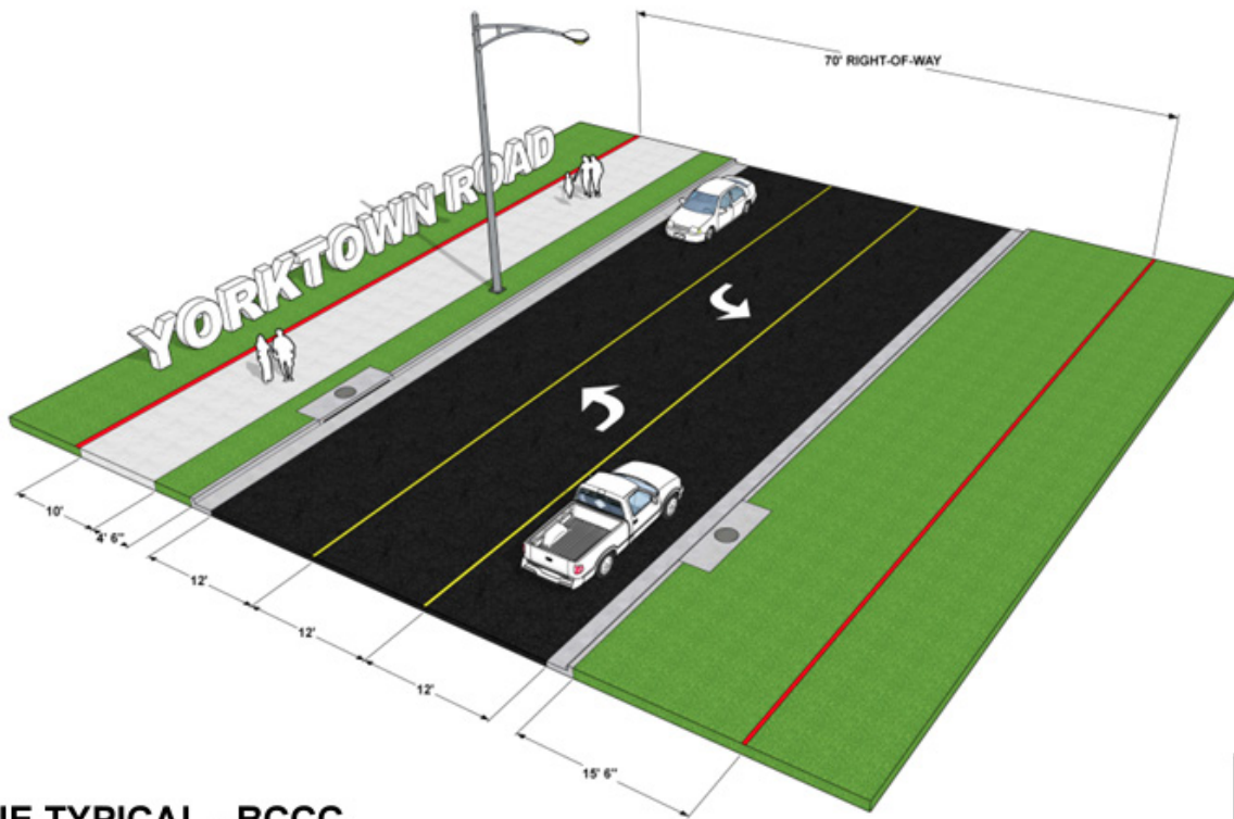
3 LANE TYPICAL - BCCC
